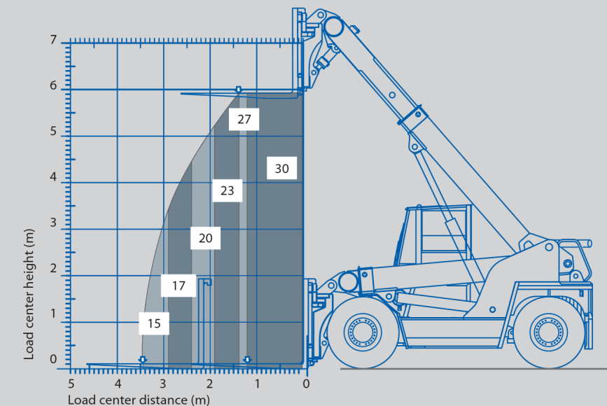
Lifting capacity diagram and working dimensions ML3012RC
