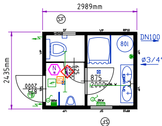
Sanitary cabin 10'
