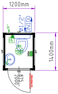
WC cabin 5'
