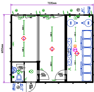
Office and sanitary cabin 3 units
