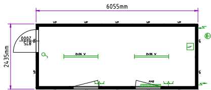
Office cabin 20' standard
