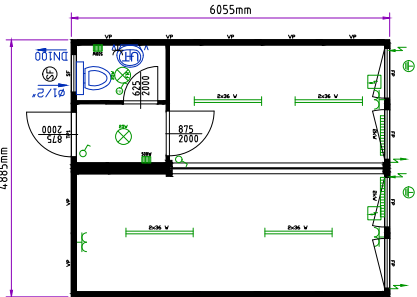
Office and sanitary cabin 2 units
