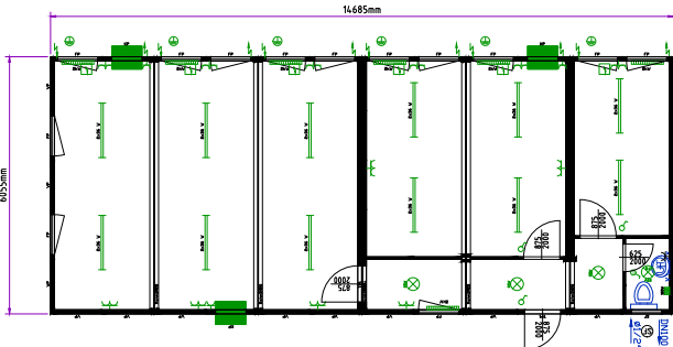
Office and sanitary cabin 6 units
