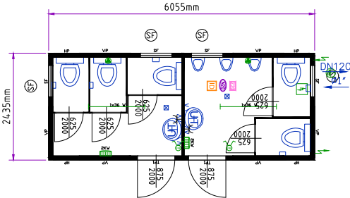
WC cabin ladies/ mens 20'
